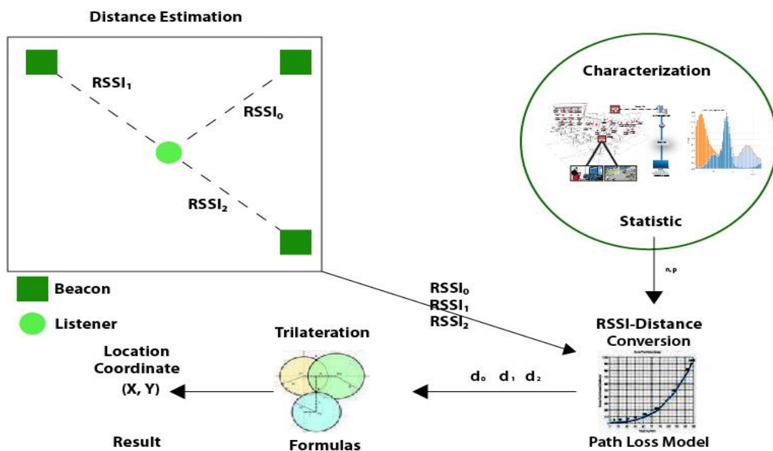
Figure 3.3: Overview simple block diagram( pu,2009 ).
